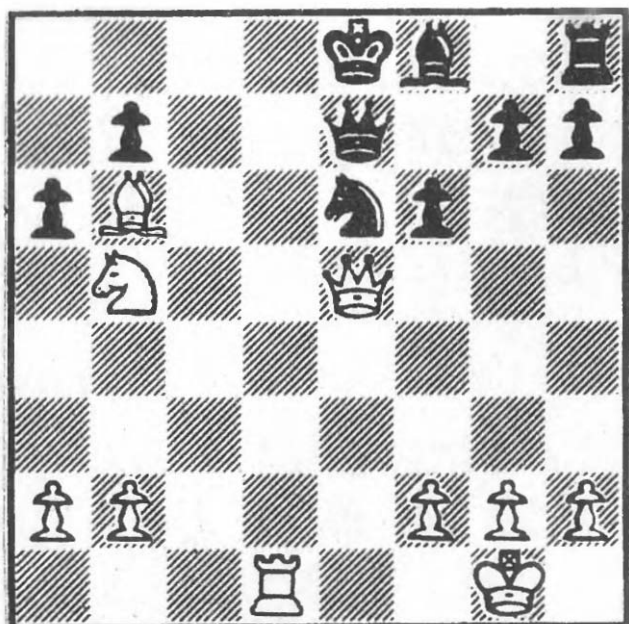
25 After 17...f6
